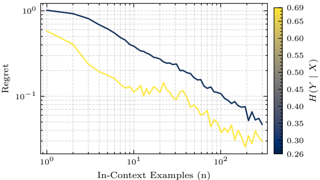
In-Context Learning Regret for Qwen-2.5 (0.5B)
